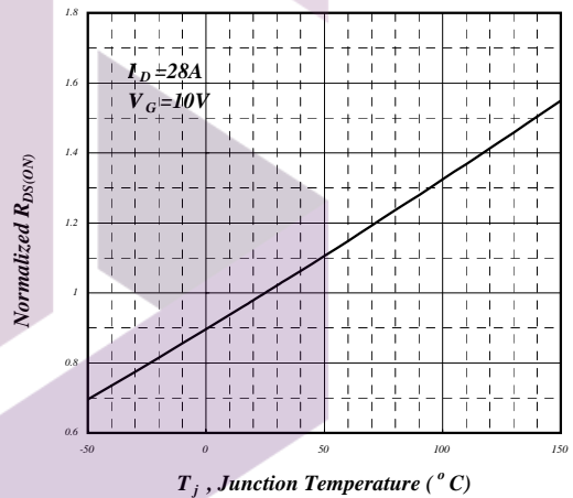
Fig 4. Normalized On-Resistance
